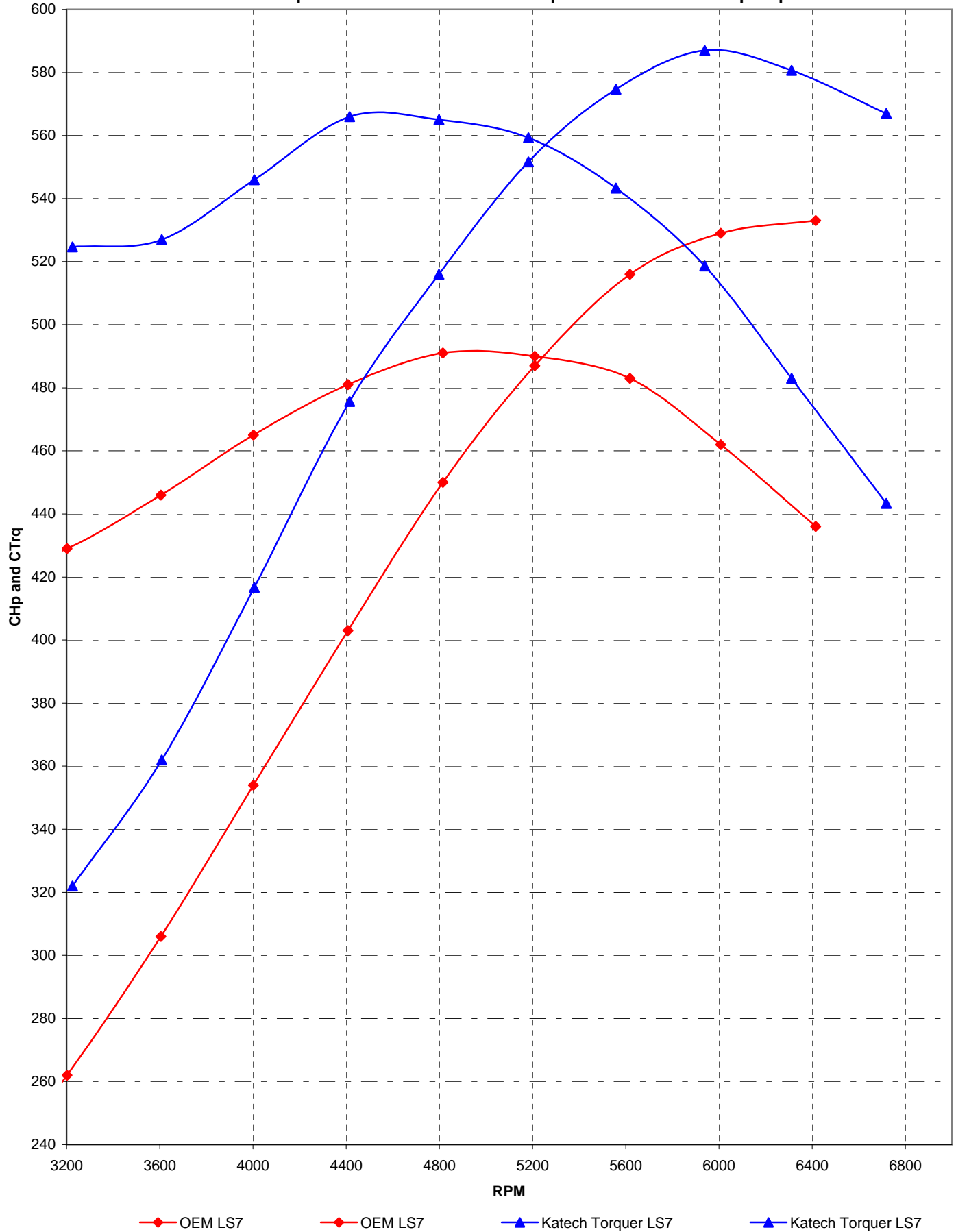
Cam Comparison - OEM Vs. Katech Torquer LS7: Corrected Trq & Hp
